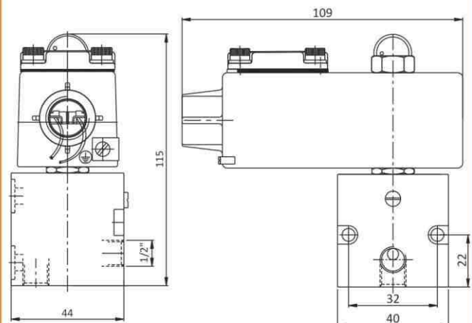
3/2 Namur Direct Acting Solenoid Valve Flame Proof / Explosion Proof Coil with CIMFR Certificate.
