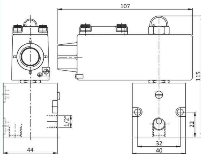
3/2 Namur Direct Acting Solenoid Valve Weather Proof with Terminal Type Junction Box Coil.
