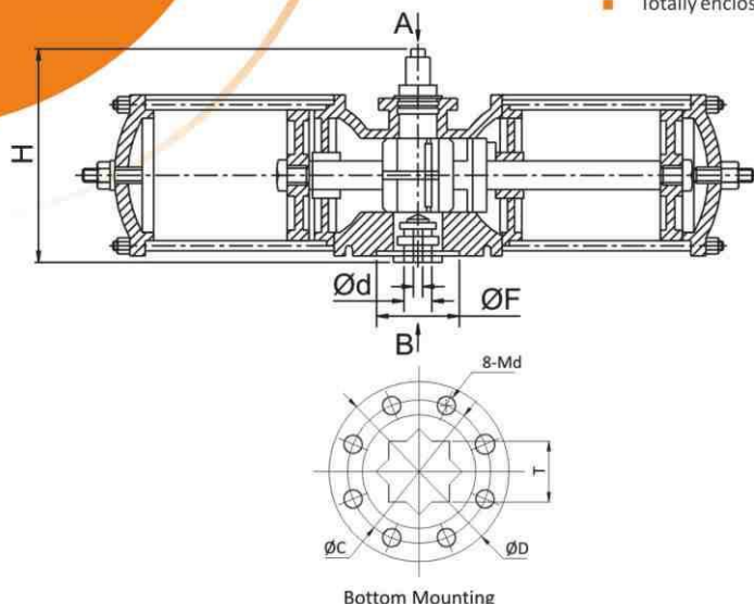
WAW 14 - WAW 35 Dimensions Table DOUBLE ACTING
