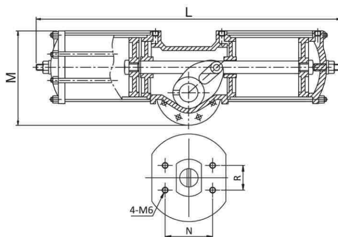
Top Mounting
