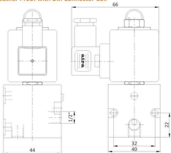
3/2 Namur Direct Acting Solenoid Valve Weather Proof with Din Connector Coil
