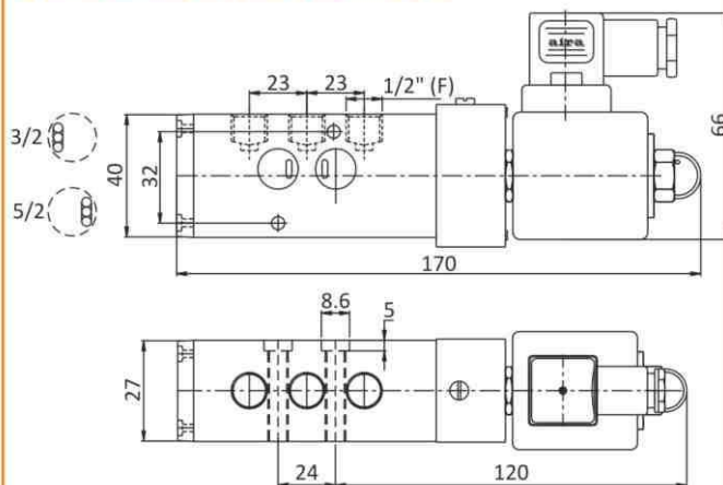
3/2 Namur Direct Acting Solenoid Valve Weather Proof with Din Connector Coil
